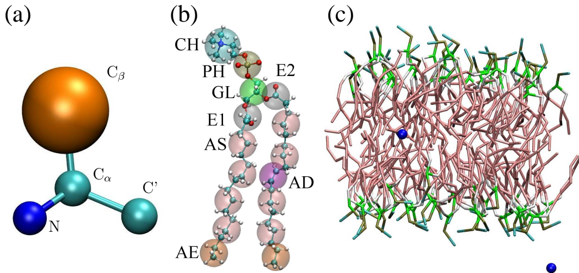
Figure 6.2: (a) Coarse-grained amino acid (colors: N dark blue, C_\alpha and C' cyan, C_\beta orange). Lipids interact with backbone bead C_\alpha and side-chain bead C_\beta . (b) Coarse-grained POPC lipid, as presented in [WD10b]. Reproduced in part with permission from Wang, Z.-J. and Deserno, M. J. Phys. Chem. B 114 (2010), no. 34, 11207–11220. Copyright 2010 American Chemical Society. (c) Side view of a 72-molecule DOPC bilayer as well as two amino acid side chains (in blue) constrained at the center and outside of the membrane.
