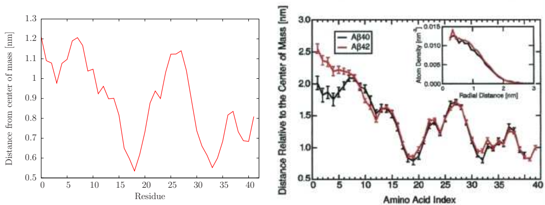
Figure 5.4: Average distance to the center of mass of the pentamer for each residue: (left) this work, conformations sampled at T = 1.0 \mathcal{E}/k_B ; (right) red curve—simulation study from Urbanc et al. [UCY + 04]. Copyright (2004) National Academy of Sciences, USA.
