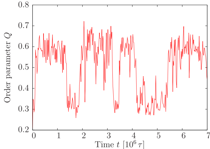
Figure 2.9: Conventional (i.e., not using parallel tempering) simulation of \alpha 3D at T = 1.2\mathcal{E}/k_B . The nativity parameter Q is plotted against time. The protein alternates between folded ( Q \gtrsim 0.6 ) and unfolded conformations ( Q \lesssim 0.5 ). Reprinted with permission from Bereau, T. and Deserno, M. J. Chem. Phys. 130 (2009), 235106 [BD09]. Copyright 2009, American Institute of Physics.
