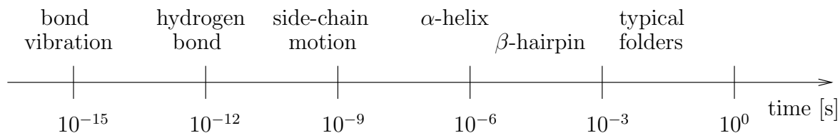
Figure 1.2: Several timescales involved in protein folding.
