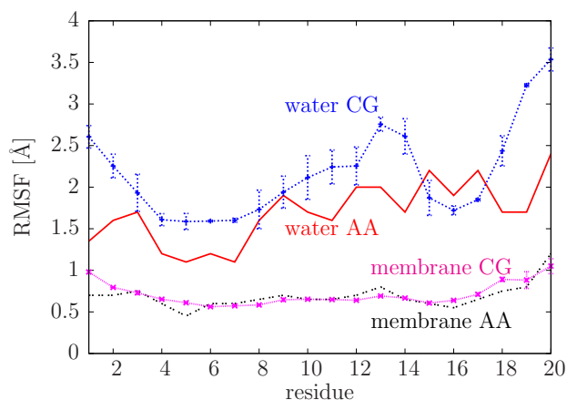
Figure 6.11: Root-mean-square fluctuations of alamethicin in water and in a POPC bilayer (denoted “membrane”). “AA” and “CG” correspond to atomistic and coarse-grained simulations, respectively. Atomistic data reproduced from Tieleman et al. [TSB99].
