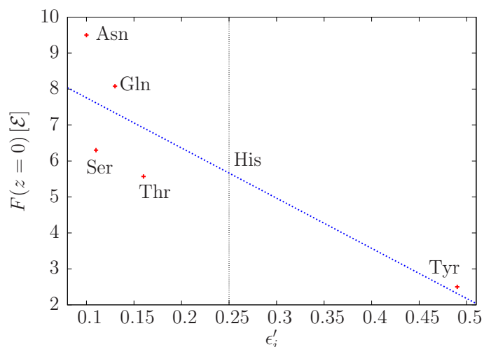
Figure 6.6: PMF height at origin F(z = 0) as a function of the normalized hydrophobicity parameter \epsilon'_i (defined in chapter 2) for several hydrophilic amino acids. PMF heights determined from the atomistic simulations of MacCallum et al. [MBT08]. Vertical line marks the hydrophobicity of histidine. Dashed line is a linear fit to the different residues. The intersection between the fit and the vertical line shows the estimate for histidine.
