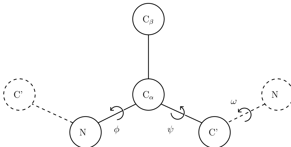
Figure 2.1: Schematic figure of the local geometry of the protein chain. The solid beads comprise one amino acid. Neighboring amino acid beads are represented in dashed lines. Reprinted with permission from Bereau, T. and Deserno, M. J. Chem. Phys. 130 (2009), 235106 [BD09]. Copyright 2009, American Institute of Physics.
