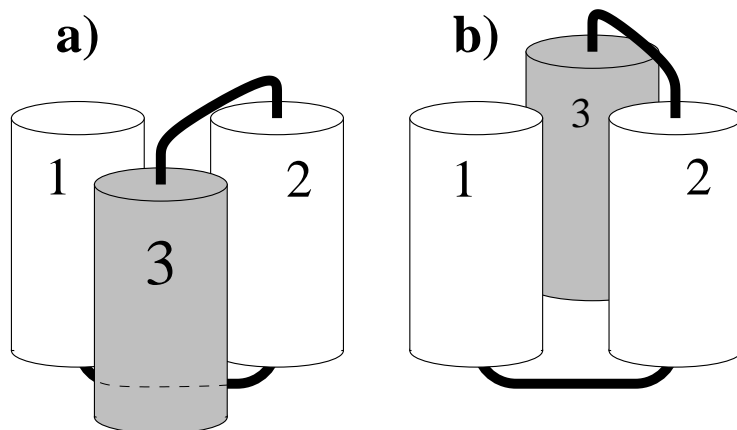
Figure 2.11: Schematic figure of the two possible topologies in forming a three-helix bundle. The native fold of protein \alpha 3D corresponds to a counterclockwise topology (a), that of GS-\alpha_3W is clockwise (b). Reprinted with permission from Bureau, T. and Deserno, M. J. Chem. Phys. 130 (2009), 235106 [BD09]. Copyright 2009, American Institute of Physics.
