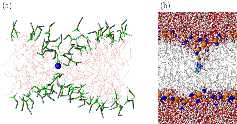
Figure 6.7: (a) Coarse-grained configuration of \text{Arg}^+ (blue sphere) in a DOPC bilayer (thin lines: hydrocarbon tails; licorice: head groups). The insertion of \text{Arg}^+ creates a strong, local deformation of the bilayer. (b) Atomistic configuration of \text{Arg}^+ in a DOPC bilayer. Reprinted from Biophysical Journal , 94 , J. L. MacCallum, W. F. D. Bennett, and D. P. Tieleman, Distribution of amino acids in a lipid bilayer from computer simulations , 3393–3404, Copyright (2008), with permission from Biophysical Society [MBT08].
