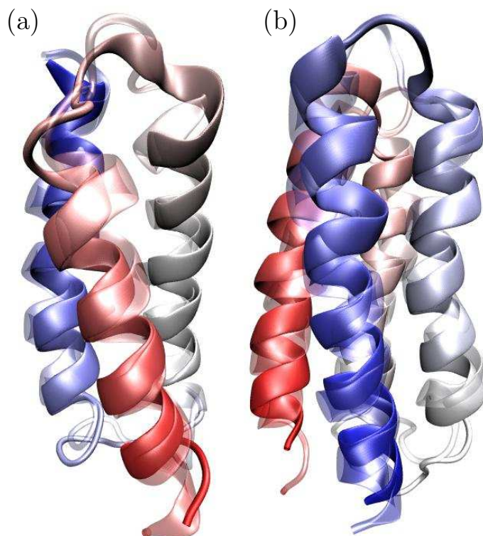
Figure 2.7: Equilibrated structures of three-helix bundle \alpha 3D (a) and four-helix bundle S-824 (b) sampled at T = 1 \mathcal{E}/k_B . Superposition of simulated structure (opaque) with experimental data (transparent) is displayed. The STRIDE algorithm [FA95] was used for secondary structure assignment (thick ribbons represent \alpha -helices on the figure). Reprinted with permission from Berau, T. and Deserno, M. J. Chem. Phys. 130 (2009), 235106 [BD09]. Copyright 2009, American Institute of Physics.
