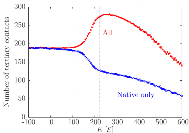
Figure 4.7: Number of tertiary contacts for \alpha 3D as a function of energy. The “All” curve (red) averages over all non-local pairs whereas the “Native only” curve (blue) only counts native pairs (see text for details). Vertical lines mark the transition region.
