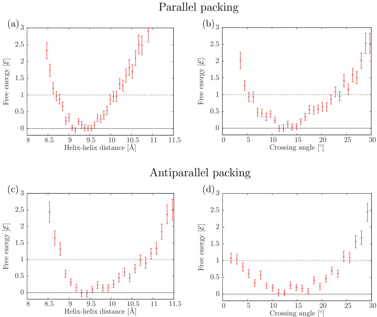
Figure 6.13: Free energies between two WALP23 peptides in a POPC bilayer as a function of the helix-helix distance, (a) and (c), and crossing angle, (b) and (d), for parallel and antiparallel packing, respectively. Horizontal lines denote F = 0 and F = 1 \mathcal{E} (i.e., thermally accessible interval). Error bars reflect the variance of the data points ( 1 \sigma interval). Helix-helix distance distributions average over all crossing angles, and vice-versa. The amount of sampling obtained here is not enough to produce two-dimensional free energy surfaces as a function of both helix-helix distance and crossing angle.
