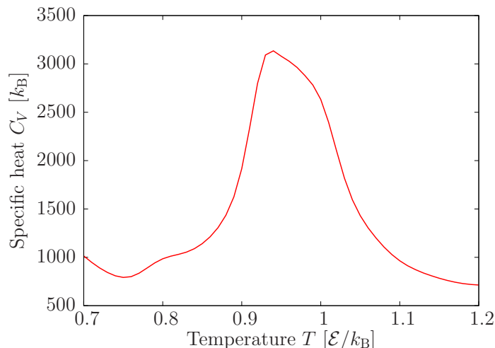
Figure 2.12: Specific heat of 15 GNNQQNY peptides in a cubic box of size 55 Å. The peak around T = 0.95 \mathcal{E}/k_B separates a low-temperature phase, rich in high- \beta content aggregates, from a high temperature phase where no aggregates form. Reprinted with permission from Bereau, T. and Deserno, M. J. Chem. Phys. 130 (2009), 235106 [BD09]. Copyright 2009, American Institute of Physics.
