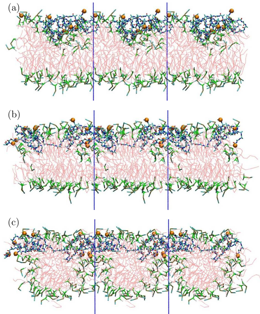
Figure 6.15: Insertion and folding of four WALP peptides on a 72-POPC lipid bilayer. Simulation snapshots recorded at t = 50\,000\tau (a), t = 450\,000\tau (b), and t = 600\,000\tau (c), respectively. Note the increasing deformation of the lower leaflet of the bilayer. Blue, vertical lines mark the periodic boundaries of the simulation box (3 identical unit cells are shown). Thin lines: lipid tails; licorice: lipid head groups and protein; orange beads: N- and C-termini.
