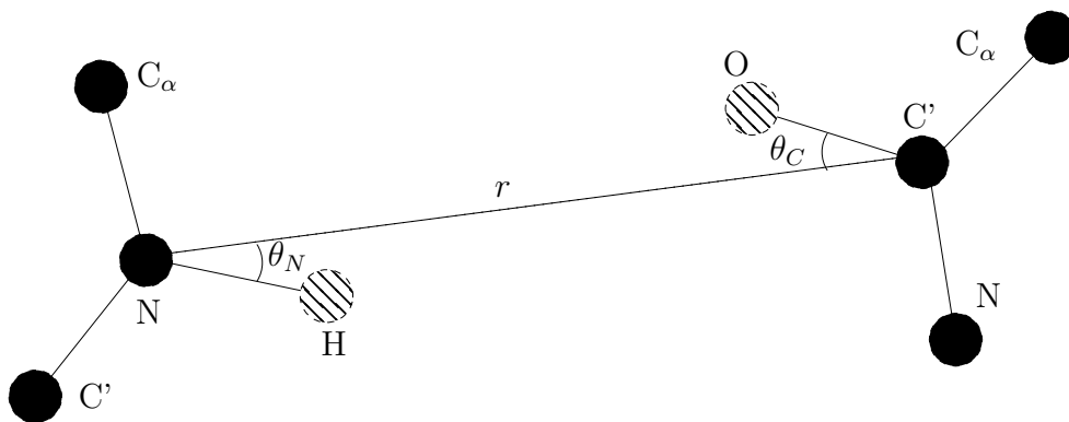
Figure 2.3: Schematic figure of the hydrogen-bond interaction. The light beads (H and O) are not explicitly modeled in the simulation; their positions are inferred from their bonded neighbors. Reprinted with permission from Berau, T. and Deserno, M. J. Chem. Phys. 130 (2009), 235106 [BD09]. Copyright 2009, American Institute of Physics.
