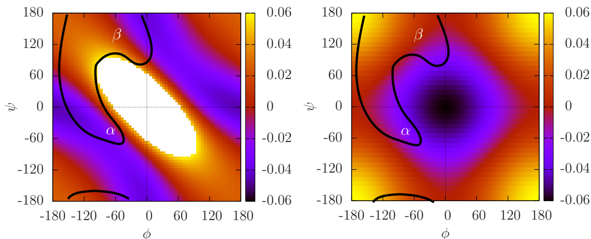
Figure 2.4: Map of the nearest-neighbor dipole-dipole interaction for all sets of dihedral angles \phi and \psi (left), and the decoupled Fourier series approximation (right). The central part of the left plot was not reproduced in order to emphasize local difference in other regions of the plot (as can be seen in Figure 2.5, this anyways is a sterically hindered region). Sterically favored regions of the plot are circumscribed by a thick line, in addition to labels of \alpha and \beta regions. The two graphs were shifted and scaled for comparison. Reprinted with permission from Bereau, T. and Deserno, M. J. Chem. Phys. 130 (2009), 235106 [BD09]. Copyright 2009, American Institute of Physics.
