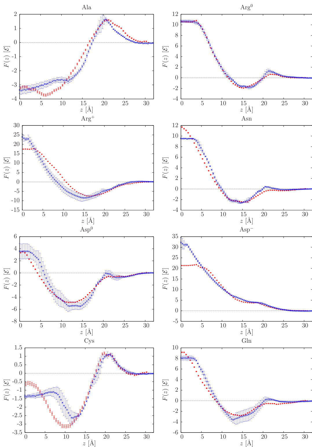
Figure 6.3: Free energy profiles for the insertion of a single amino acid in a DOPC bilayer: coarse-grained (red, solid) and atomistic (blue, dashed. From MacCallum et al. [MBT08].). Part 1/3.
