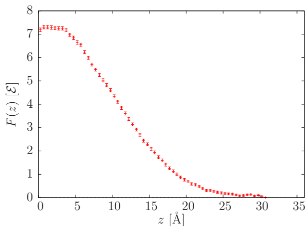
Figure 6.10: Free energy profile for the insertion of a coarse-grained N- or C-terminus side chain in a DOPC bilayer.
