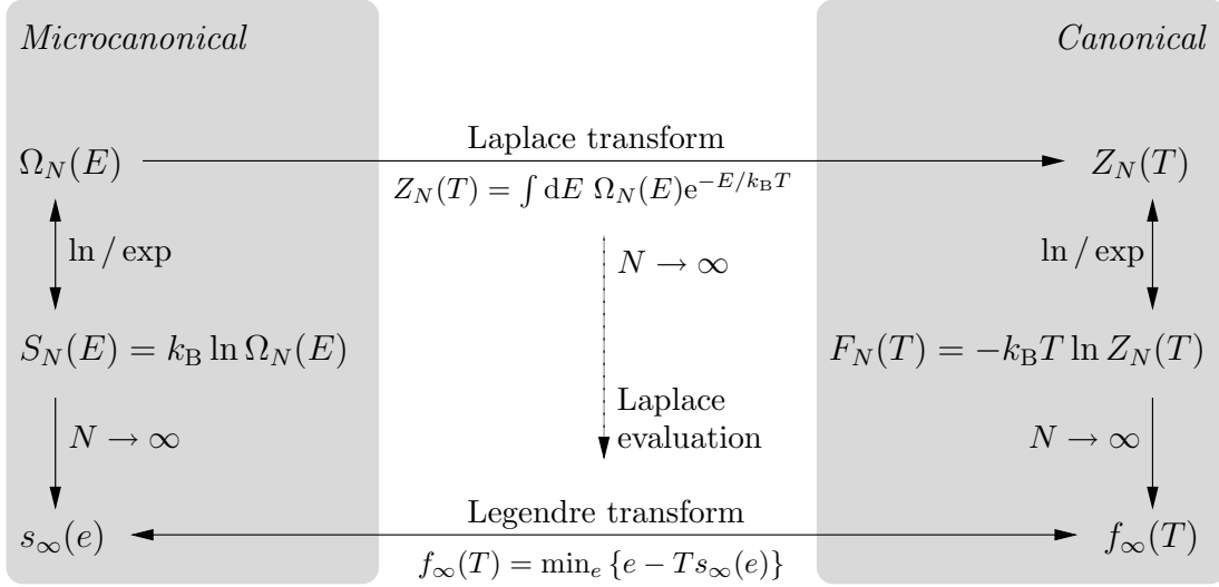
Figure 4.2: Thermodynamic quantities in the microcanonical (left) and canonical (right) ensembles. Arrow heads denote how quantities can be determined from others. For instance, the density of states determines the partition function but not the other way around (numerically, at least). For more details, see main text.
