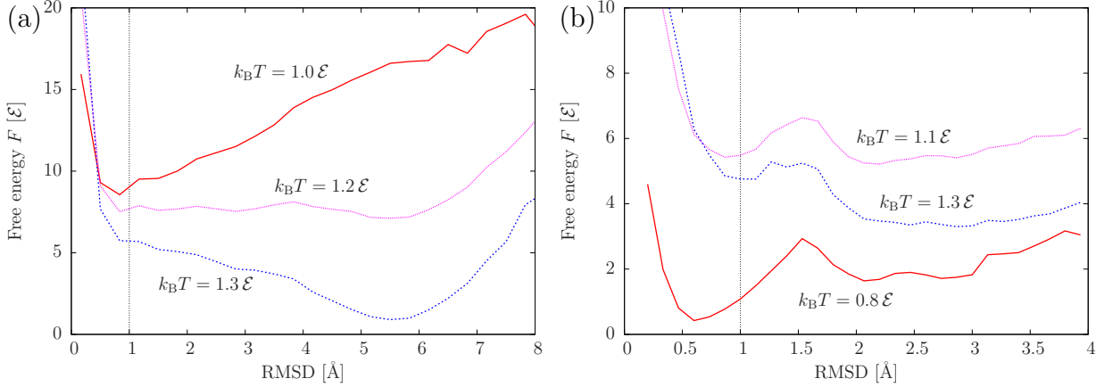
Figure 3.2: Free energy as a function of the RMSD from the sampled structure with lowest potential energy for (a) (AAQAA)_3 and (b) V_5^D P G V_5 . The three curves represent the free energy at temperature T = \{1.0, 1.2, 1.3\} \mathcal{E}/k_B and T = \{0.8, 1.1, 1.3\} \mathcal{E}/k_B , respectively. The vertical line indicates a 1 \text{ \AA} RMSD used as the folding threshold in section 3.2.
