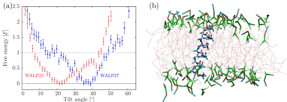
Figure 6.12: (a) Free energy as a function of tilt angle for WALP23 (red) and WALP27 (blue) in POPC. Horizontal lines denote F = 0 and F = 1 \mathcal{E} (i.e., thermally accessible interval). Error bars reflect the variance of the data points ( 1 \sigma interval). (b) Representative conformation of WALP23 (thin lines: lipid tails; licorice: lipid head groups and protein).
