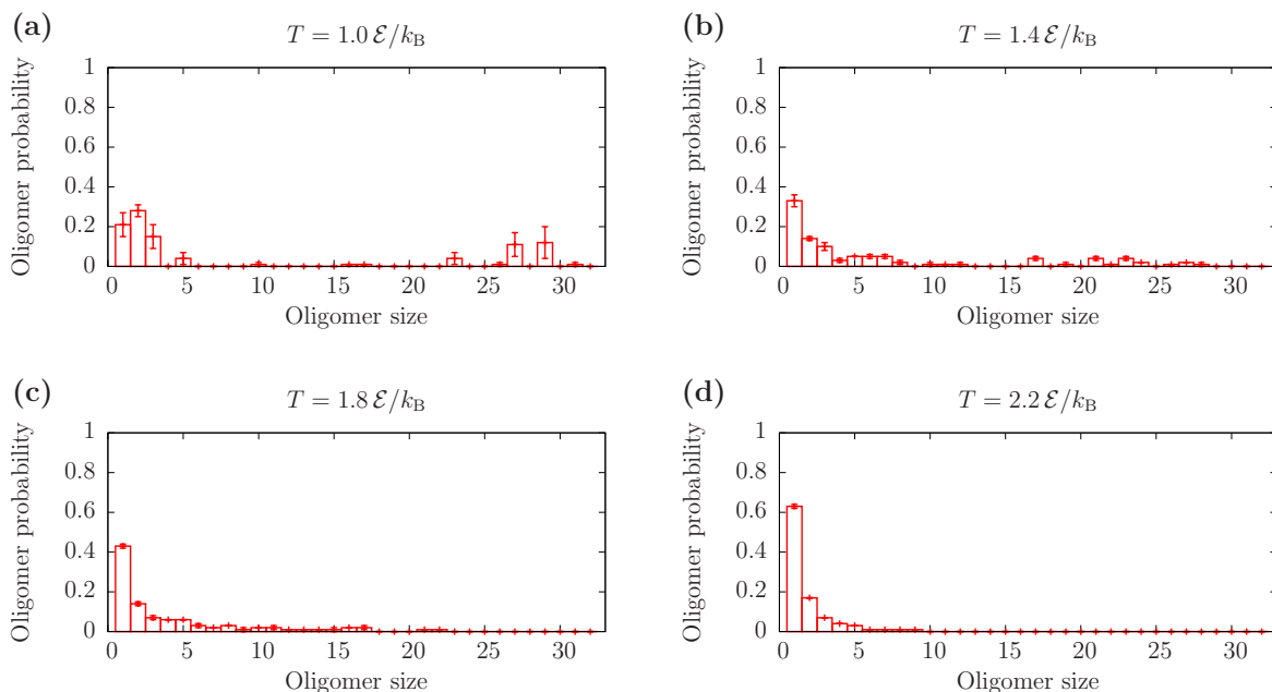
Figure 5.2: Oligomer distribution functions of a system of 32 A\beta_{1-42} at temperatures (a) T = 1.0 \mathcal{E}/k_B , (b) T = 1.4 \mathcal{E}/k_B , (c) T = 1.8 \mathcal{E}/k_B , and (d) T = 2.2 \mathcal{E}/k_B .
