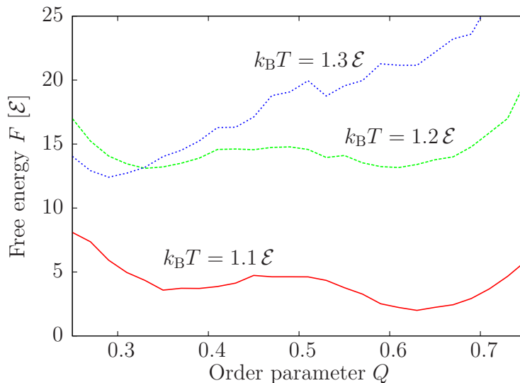
Figure 2.8: Free energy profile as a function of nativeness order parameter Q (Equation 2.16) below ( T = 1.1 \mathcal{E}/k_B ), at, and above ( T = 1.3 \mathcal{E}/k_B ) the folding temperature T_f = 1.2 \mathcal{E}/k_B for \alpha 3D . Reprinted with permission from Bereau, T. and Deserno, M. J. Chem. Phys. 130 (2009), 235106 [BD09]. Copyright 2009, American Institute of Physics.
