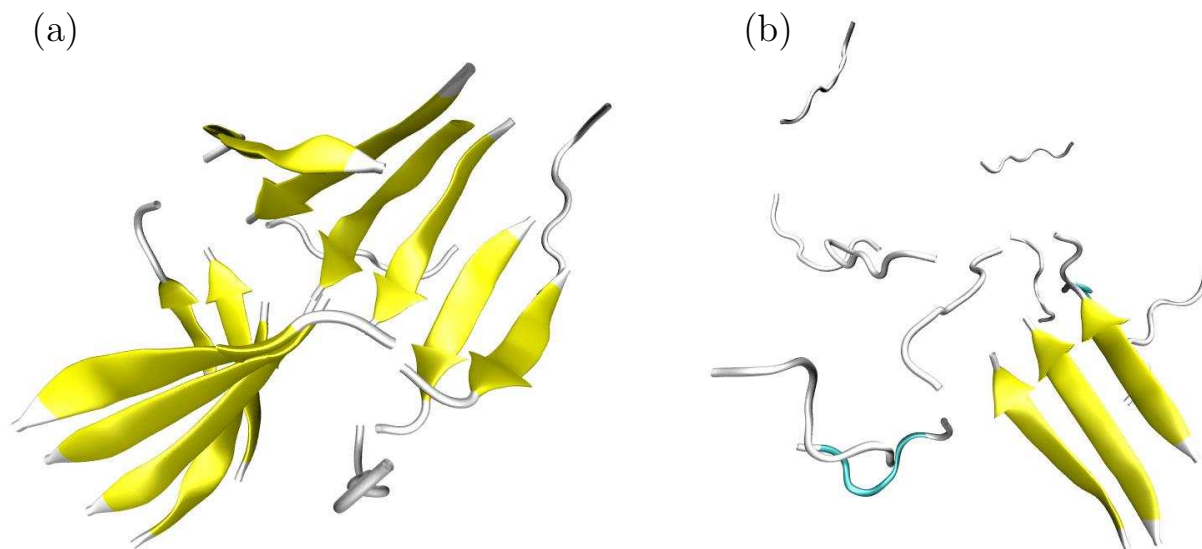
Figure 2.13: Snapshot of representative conformations at: (a) T = 0.8 \mathcal{E}/k_B where peptides aggregate into a condensed phase and (b) T = 1.0 \mathcal{E}/k_B which mostly samples disordered monomers. These two temperatures are located on both sides of the system's transition, as shown in Figure 2.12. Reprinted with permission from Bereau, T. and Deserno, M. J. Chem. Phys. 130 (2009), 235106 [BD09]. Copyright 2009, American Institute of Physics.
