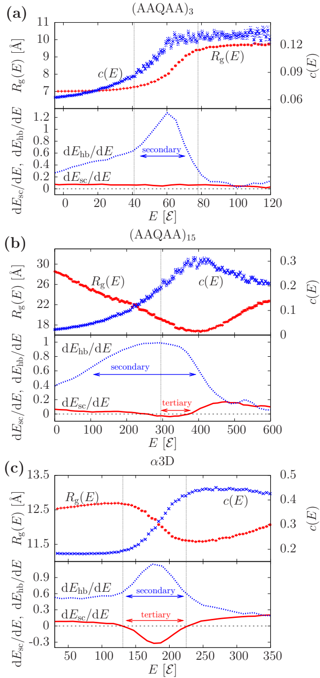
Figure 4.6: (top) Radius of gyration R_g(E) (red) and normalized acylindricity parameter c(E) (blue), both with the error of the mean, as well as (bottom) rates of hydrogen-bond and side-chain energies dE_{hb}/dE and dE_{sc}/dE , respectively, for (a) (AAQAA)_3 , (b) (AAQAA)_{15} , and (c) \alpha 3D . Vertical lines mark either the transition region ( n = 3 , \alpha 3D ) or the transition point ( n = 15 ).
