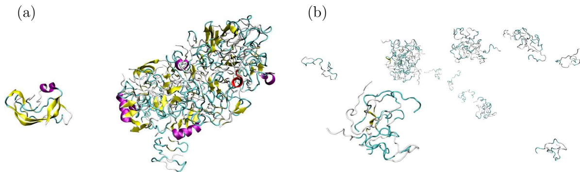
Figure 5.1: Conformations of a system of 32 A\beta_{1-42} sampled at (a) T = 1.0 \mathcal{E}/k_B and (b) T = 2.2 \mathcal{E}/k_B .
