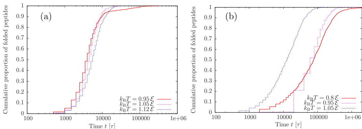
Figure 3.3: Cumulative proportion of folded peptides as a function of time for (a) (\text{AAQAA})_3 and (b) \text{V}_5^{\text{D}}\text{PGV}_5 at different temperatures. Right boundaries correspond to the maximum simulation time.
