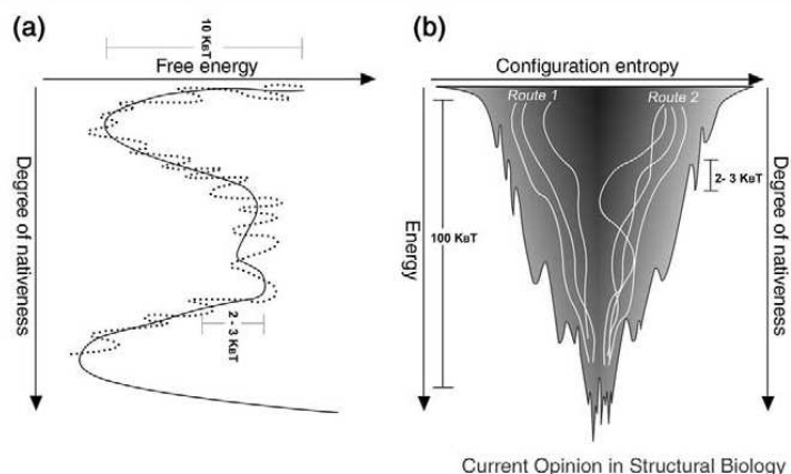
Figure 1.1: Cartoon of the folding energy landscape is shown in (b). This illustrates the competition between few low-energy, low-entropy folds (bottom; folded) with a large number of high-energy, high-entropy conformations (top; unfolded). The ruggedness of the landscape suggests the existence of kinetic traps. On the left (a), the corresponding free energy as a function of a valid order parameter (i.e., one that can describe the evolution of the system) shows two minima: one at high energy, high entropy (unfolded) and the other at low energy, low entropy (folded). Reprinted from Current Opinion in Structural Biology , 14 , J. N. Onuchic and P. G. Wolynes, Theory of protein folding , 70–75 [OW04], Copyright (2004), with permission from Elsevier.
