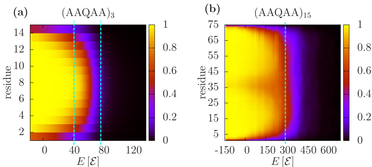
Figure 4.4: Amount of secondary structure as a function of energy and residue for (a) (AAQAA)_3 and (b) (AAQAA)_{15} . Vertical lines mark the transition region (a) and point (b), respectively.
