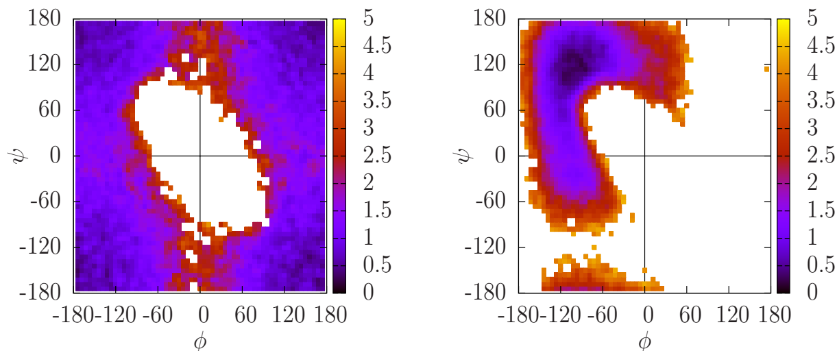
Figure 2.5: Free energy plots of tripeptides Gly-Gly-Gly (left) and Gly-Ala-Gly (right), as a function of successive dihedrals \phi and \psi , calculated at our reference temperature T = 1 \text{ } \mathcal{E}/k_{\text{B}} . The coloring represents the free energy difference with the lowest conformation, in units of k_{\text{B}}T . Reprinted with permission from Berau, T. and Deserno, M. J. Chem. Phys. 130 (2009), 235106 [BD09]. Copyright 2009, American Institute of Physics.
