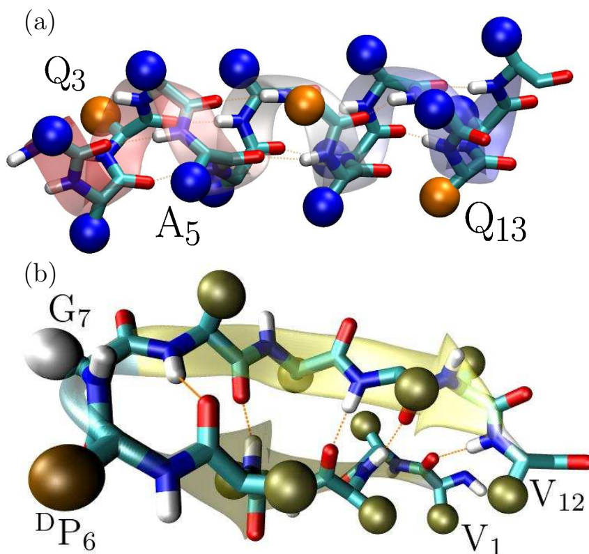
Figure 3.1: CG snapshots of the folded conformations of (a) \alpha -helix (AAQAA) 3 sampled at T = 1.0 \mathcal{E}/k_B and (b) \beta -hairpin V 5 D PGV 5 sampled at T = 0.7 \mathcal{E}/k_B . Labels indicate amino acid names with their sequence position. The larger beads represent side chains and the light dashed lines show hydrogen bonds. Rendering was done with VMD [HDS96].
