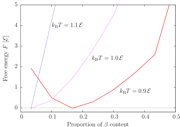
Figure 2.14: Free energy as a function of the (normalized) amount of \beta content for 15 GNNQQNY peptides at temperatures T = \{0.9, 1.0, 1.1\} \mathcal{E}/k_B . All curves were shifted vertically such that F = 0 corresponds to the lowest free energy. The horizontal shift (i.e., the first data points are away from zero) is due to the binning of the order parameter upon calculating F .
