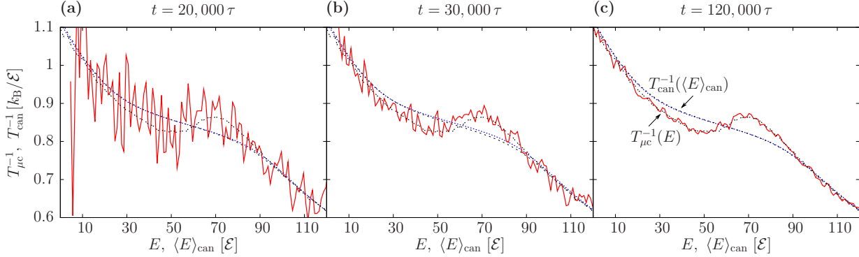
Figure 4.1: Convergence of microcanonical and canonical descriptions. Inverse temperature as a function of energy from canonical ( T_{\text{can}}^{-1}(\langle E_{\text{can}} \rangle) , blue) and microcanonical ( T_{\mu\text{c}}^{-1} = \partial S / \partial E , red) descriptions, where \langle E_{\text{can}} \rangle is the canonical average energy. Averages calculated over simulation times t = 20\,000 \tau (left), t = 30\,000 \tau (middle), and t = 120\,000 \tau (right). In each case, the black curves correspond to canonical and microcanonical averages calculated over a simulation time t = 10^6 \tau , also reproduced in Figure 4.3 (a). While canonical averages converge rapidly (the canonical blue and black curves are indistinguishable at t = 20\,000 \tau ) to a monotonic—and rather uninteresting—curve, the slower convergence of the corresponding microcanonical curves finally provides a back-bending effect—a clear indicator of first-order transition (see main text).
