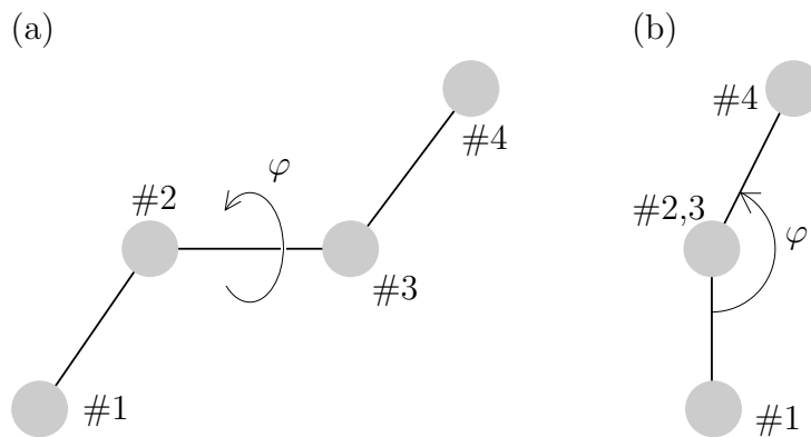
Figure 2.2: Schematic figure of the convention used when measuring a dihedral \varphi from the four beads #1,2,3,4. Side view (a) and view along the vector from bead #2 to bead #3 (b).
