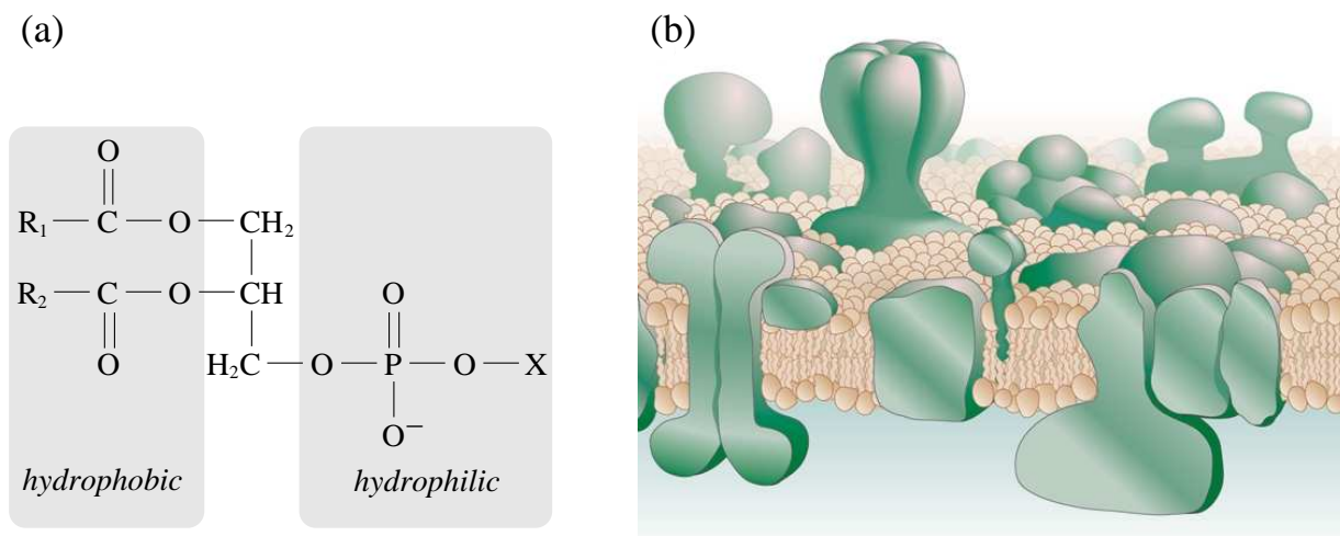
Figure 6.1: (a) Chemical representation of a phospholipid molecule. Fatty acid chains (denoted R_1 and R_2 ) form the hydrophobic region of the molecule. The hydrophilic region is composed of a phosphate group and a head group (denoted X; e.g., serine, choline, glycerol). An atomistic representation of a phosphatidylcholine lipid is displayed in Figure 6.2. (b) Cartoon representation of a cell membrane composed of lipid molecules (beige) crowded by many integral and peripheral proteins (green inclusions). Adapted by permission from Macmillan Publishers Ltd: Nature 438 , 578–580 (1 December 2005), copyright 2005 [Eng05].
