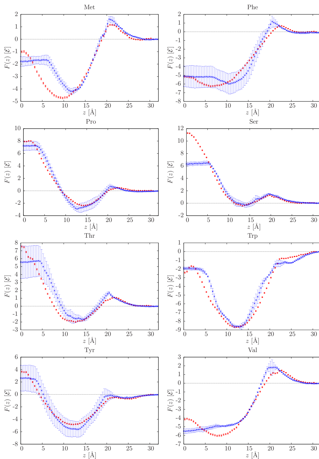
Figure 6.5: Free energy profiles for the insertion of a single amino acid in a DOPC bilayer: coarse-grained (red, solid) and atomistic (blue, dashed). From MacCallum et al. [MBT08]. Part 3/3. Reference data for Pro were extrapolated as described in the text.
