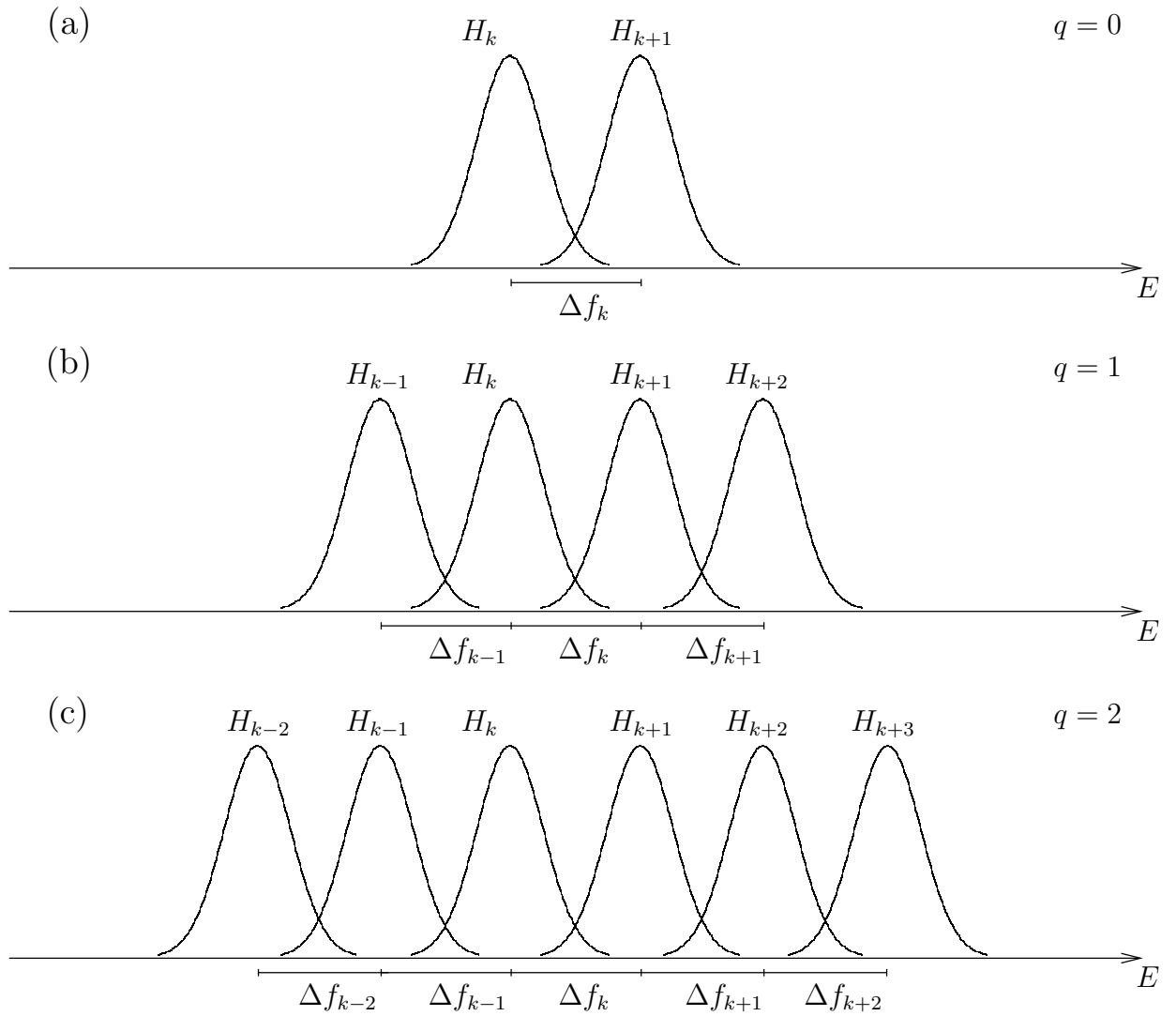
Figure A.1: Iterative refinement of the free energy difference \Delta f_k for (a) q = 0 which corresponds to the original Bennett equation (Equation A.18), (b) q = 1 , and (c) q = 2 , corresponding to one and two additional histograms on each side, respectively.
