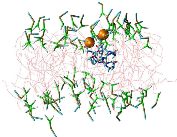
Figure 6.14: Insertion and folding of one WALP peptides on a 72-POPC lipid bilayer. Simulation snapshots recorded at t = 1.5 \times 10^6 \tau . Thin lines: lipid tails; licorice: lipid head groups and protein; orange beads: N- and C-termini.
