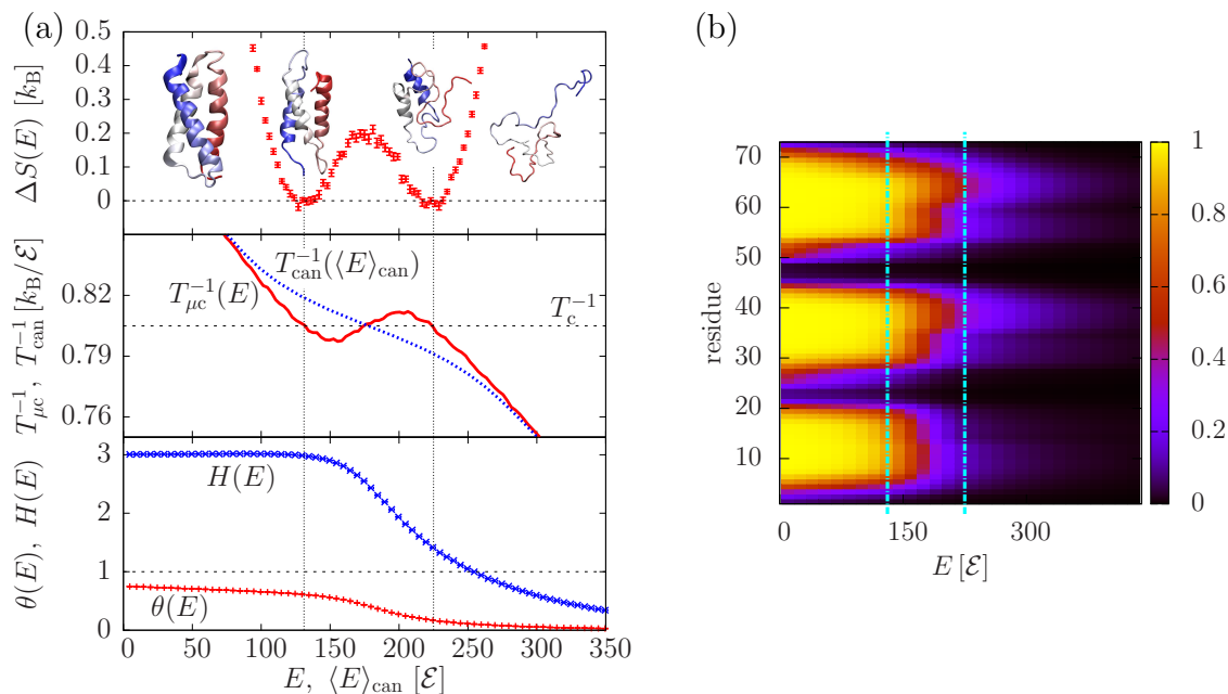
Figure 4.5: Three-helix bundle \alpha 3D. (a) From top to bottom: \Delta S(E) , error bars reflect the variance of the data points ( 1\sigma interval); inverse temperatures from canonical ( T_{\text{can}}^{-1}(\langle E_{\text{can}} \rangle) , blue) and microcanonical ( T_{\mu\text{c}}^{-1} = \partial S / \partial E , red) descriptions, where \langle E_{\text{can}} \rangle is the canonical average energy; helicity \theta(E) (red) and number of helices H(E) (blue), both with the error of the mean. Vertical lines delimit the transition region. Representative conformations at different energies are shown. (b) Amount of secondary structure as a function of energy and residue. Vertical lines mark the transition region.
