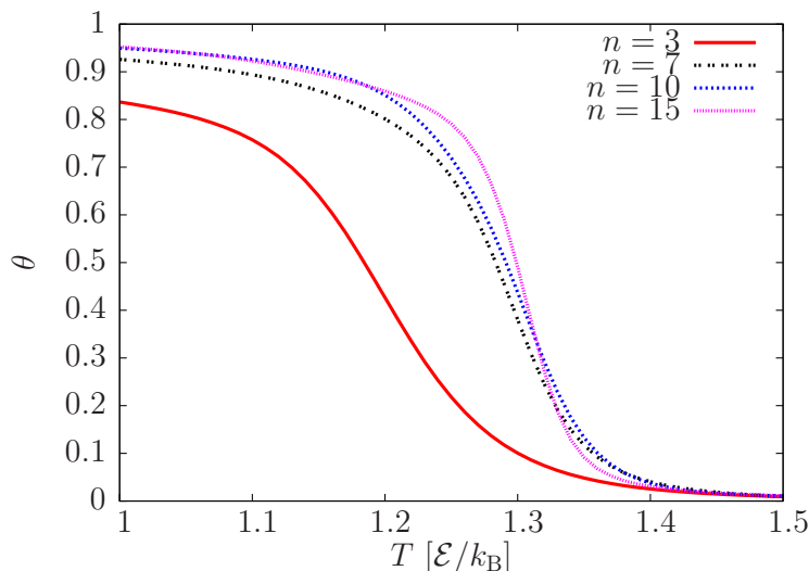
Figure 4.9: Canonical helicity \theta(T) for (AAQAA)_n , n \in \{3, 7, 10, 15\} . The transition becomes sharper for longer chains.
