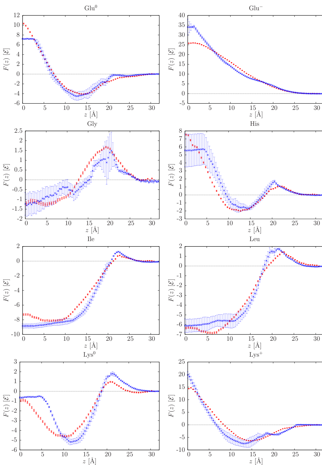
Figure 6.4: Free energy profiles for the insertion of a single amino acid in a DOPC bilayer: coarse-grained (red, solid) and atomistic (blue, dashed). From MacCallum et al. [MBT08]. Part 2/3. Reference data for Gly and His were extrapolated as described in the text.
