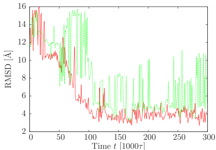
Figure 2.6: RMSD of the CG protein \alpha 3D (full line) and S-824 (dashed line) compared with experimentally resolved structures. Both simulations were run at T = 1\mathcal{E}/k_B . Reprinted with permission from Bereau, T. and Deserno, M. J. Chem. Phys. 130 (2009), 235106 [BD09]. Copyright 2009, American Institute of Physics.
