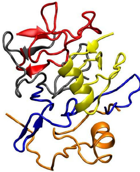
Figure 5.3: Sampled (but not necessarily representative) conformation of an A\beta_{1-42} pentamer at T = 1.0 \mathcal{E}/k_B .
