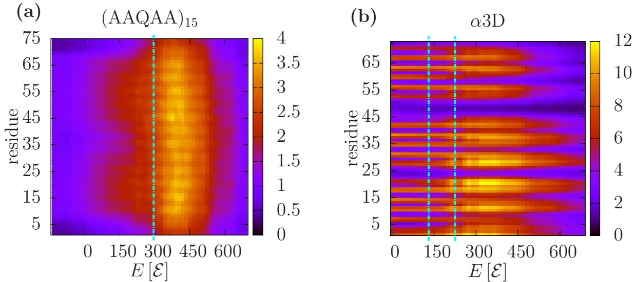
Figure 4.8: Number of tertiary contacts as a function of energy and residue for (a) (AAQAA)_{15} and (b) \alpha 3D . The two plots have different depth ranges. Vertical lines mark the transition point (a) and region (b).
