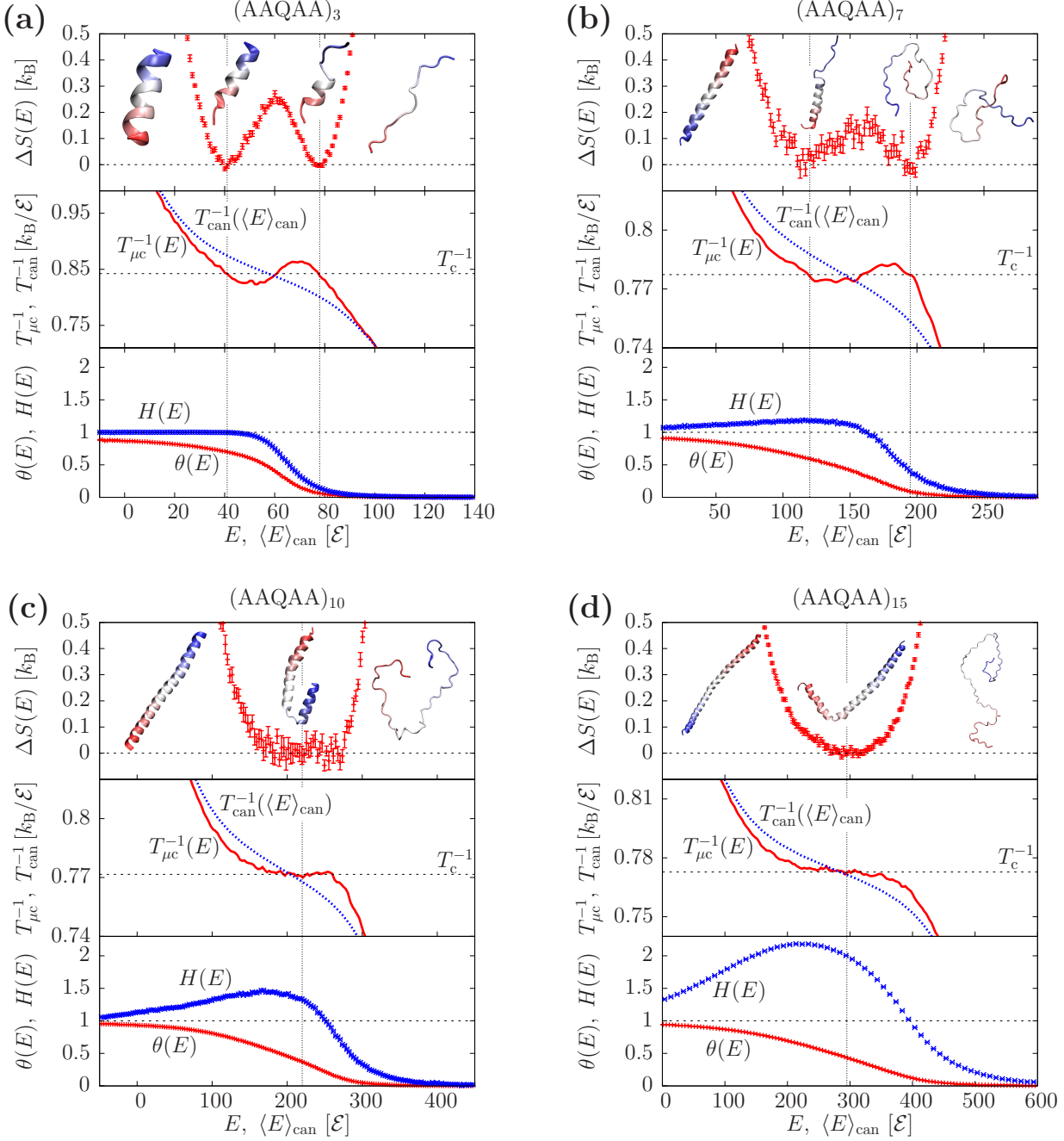
Figure 4.3: (AAQAA)_n for different chain lengths: (a) n = 3 , (b) n = 7 , (c) n = 10 , (d) n = 15 . From top to bottom for each inset: \Delta S(E) , error bars reflect the variance of the data points ( 1\sigma interval); inverse temperatures from canonical ( T_{\text{can}}^{-1}(\langle E_{\text{can}} \rangle) , blue) and microcanonical ( T_{\mu c}^{-1} = \partial S / \partial E , red) descriptions, where \langle E_{\text{can}} \rangle is the canonical average energy; helicity \theta(E) (red) and number of helices H(E) (blue), both with the error of the mean. Vertical lines mark either the transition region ( n = 3, 7 ) or the transition point ( n = 10, 15 ). Representative conformations at different energies are shown.
