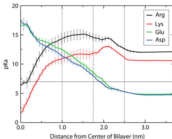
Figure 6.8: pK_a of ionizable residues as a function of bilayer depth z . pK_a values at large z (bulk water) correspond to the values reported in Table 1.2. Reprinted from Biophysical Journal, 94 , J. L. MacCallum, W. F. D. Bennett, and D. P. Tieleman, Distribution of amino acids in a lipid bilayer from computer simulations , 3393–3404, Copyright (2008), with permission from Biophysical Society [MBT08].
