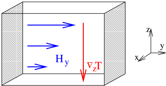
FIG. 1: Shear excitation u_{xz} in a ferrogel due to applied temperature oscillations along the z direction, in the presence of a constant or gradient magnetic field in y direction.
