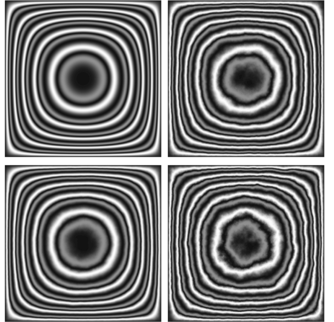
FIG. 2: The pattern at time 0.1 t_0 for a square cell (500 by 500 grid points) is shown as a function of the applied noise strength \xi_0 , which is 0 , 8\omega_L (left column), 16\omega_L , and 24\omega_L (right column). Note that \xi_0^2 \Delta^2 \Delta_t is the relevant parameter for noise, e.g., decreasing \Delta by some factor one must increase \xi_0 by the same factor for an equal noise effect, provided that \Delta is small compared to all other physical length scales (analogously for \Delta_t ).
