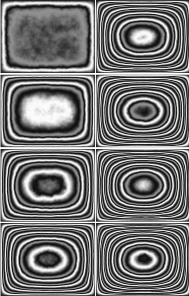
FIG. 1: Time evolution of the simulated phase winding pattern with noise (noise amplitude \xi_0 = 10\omega_L ) under the reflecting-polarizing microscope. The system is rectangular with aspect ratio 1.3 (according to 650 by 500 grid points); the director is horizontal ( \Phi = 0 ) initially. We show plots from top (left column) at times 0.01 t_0 , 0.03 t_0 , 0.05 t_0 , 0.07 t_0 , and (right column) 0.09 t_0 , 0.11 t_0 , 0.13 t_0 , and 0.15 t_0 . The gray scale in this and the following figures was calculated using the dependence of the reflectivity on the director orientation given in Ref.[7].
